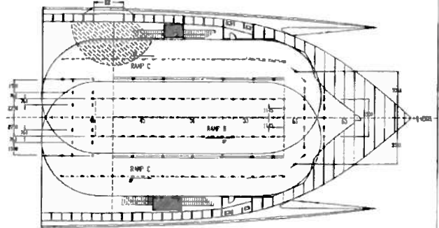
RAMPS B AND C
