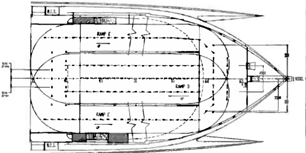
TIER 2/RAMPS D AND E
