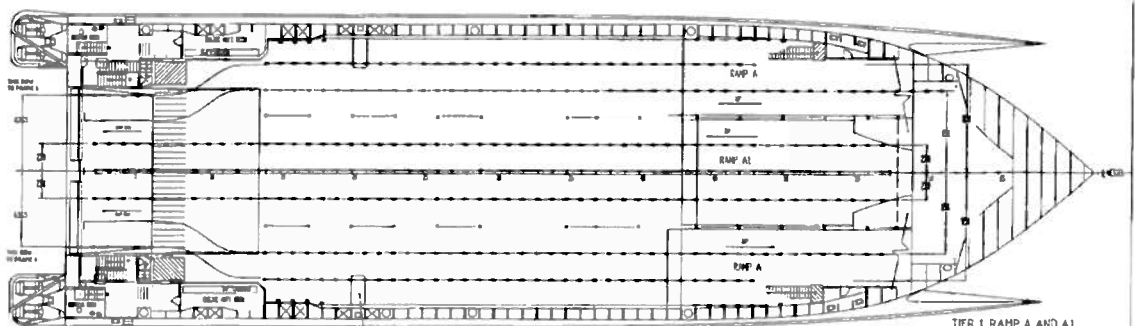
TIER 1, RAMP A AND A1
